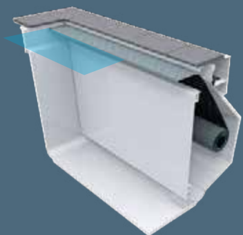
The niche extends the pool by approx. 35 cm, reducing the swimming length by approx. 50 cm.
